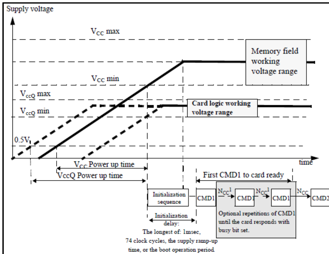
Figure 6.2 eMMC Power-Up Diagram
