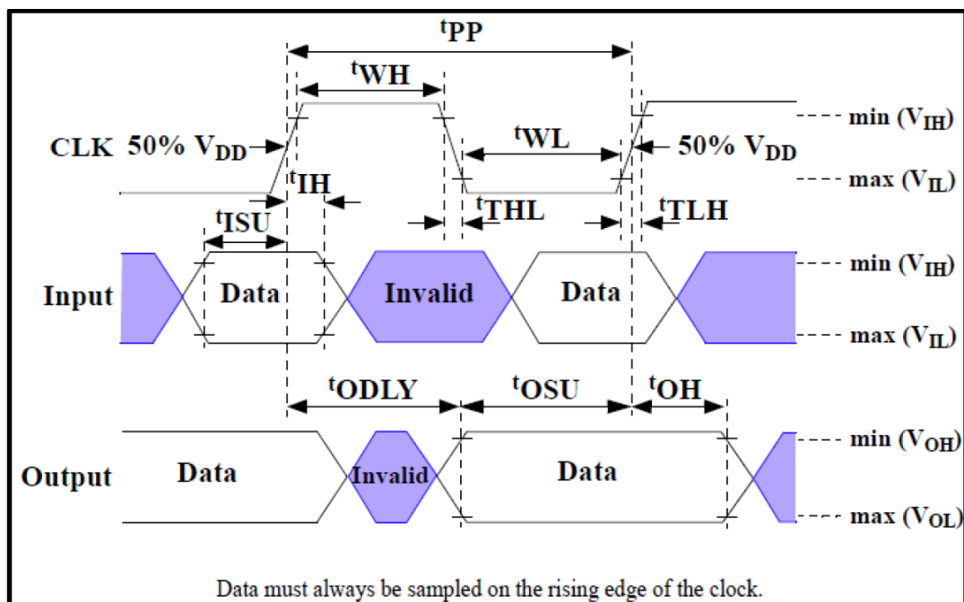
Figure 6.7 – Timing Diagram
