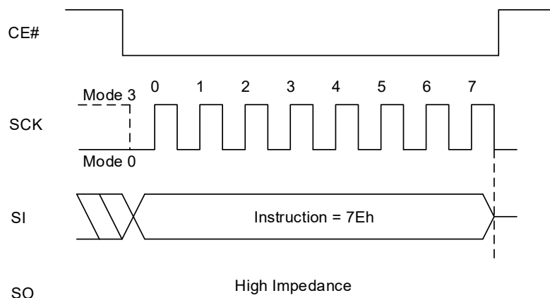
Figure 8.141 Gang Sector/Block Lock Sequence In SPI Mode
