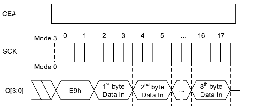
Figure 8.140 Unlock Password Sequence In QPI Mode
