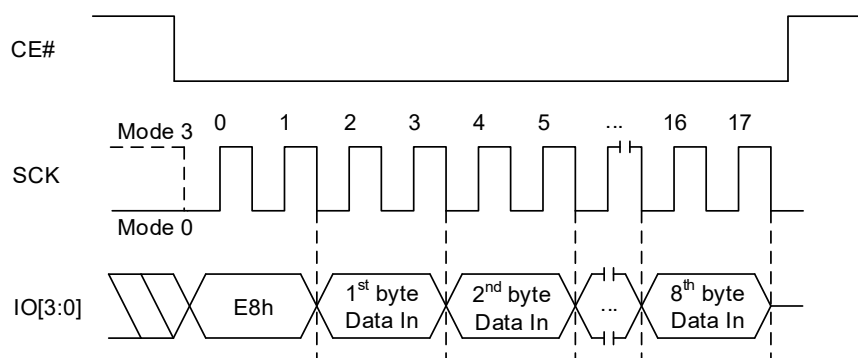
Figure 8.138 Program Password Sequence In QPI Mode
