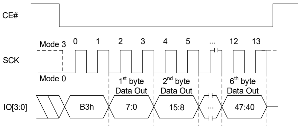
Figure 8.157 Read ECC Register In QPI Mode
