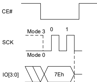
Figure 8.142 Gang Sector/Block Lock Sequence In QPI Mode
