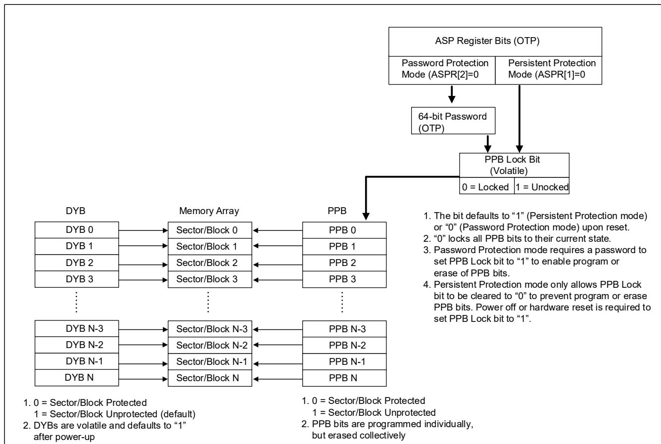
Figure 7.1 Advanced Sector/Block Protection when block size is 64KB
