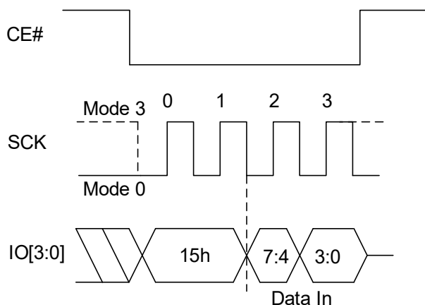
Figure 8.161 Write ECC Register Sequence In QPI Mode
