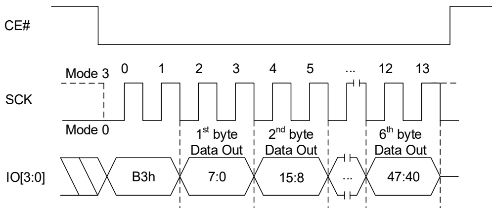
Figure 8.157 Read ECC Register In QPI Mode
