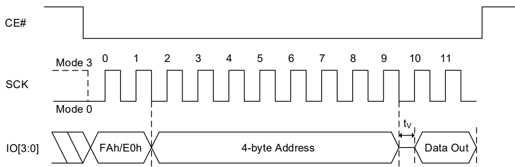
Figure 8.108 Read DYB Sequence In QPI Mode (FAh [EXTADD=0] or E0h, 4-byte address)
