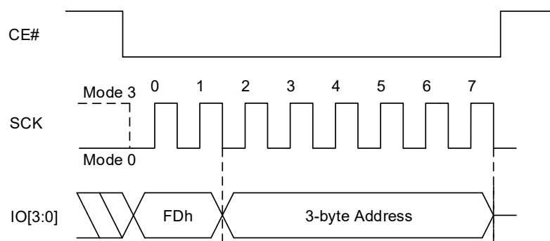
Figure 8.117 Program PPB Sequence In QPI Mode (FDh [EXTADD=0], 3-byte address)
