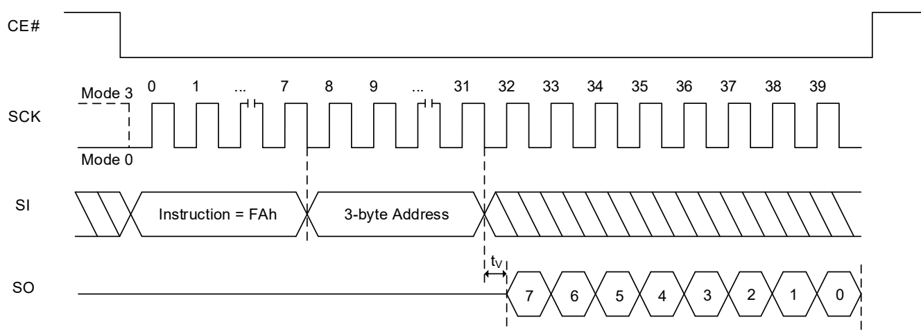
Figure 8.105 Read DYB Sequence In SPI Mode (FAh [EXTADD=0], 3-byte address)
