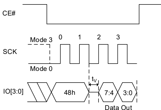
Figure 8.51 Read Function Register QPI Sequence
