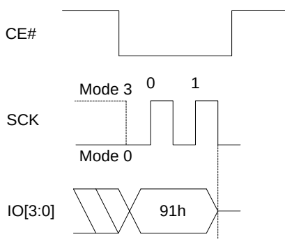
Figure 8.130 Set FREEZE Bit Sequence In QPI Mode
