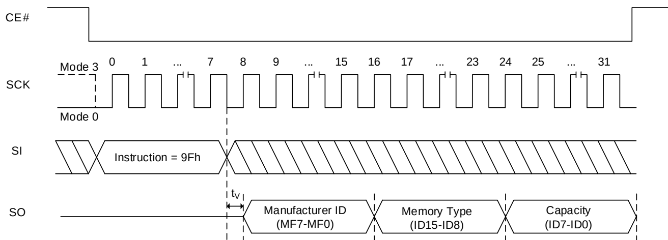
Figure 8.72 Read Product Identification by JEDEC ID Read Sequence in SPI mode
