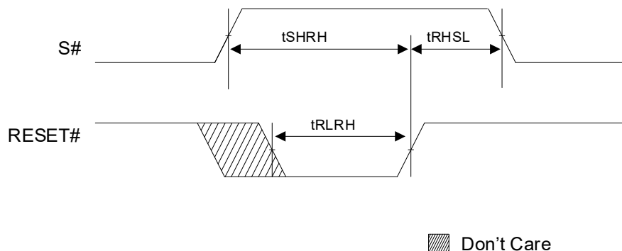
Figure 9.3 SERIAL INPUT TIMING
