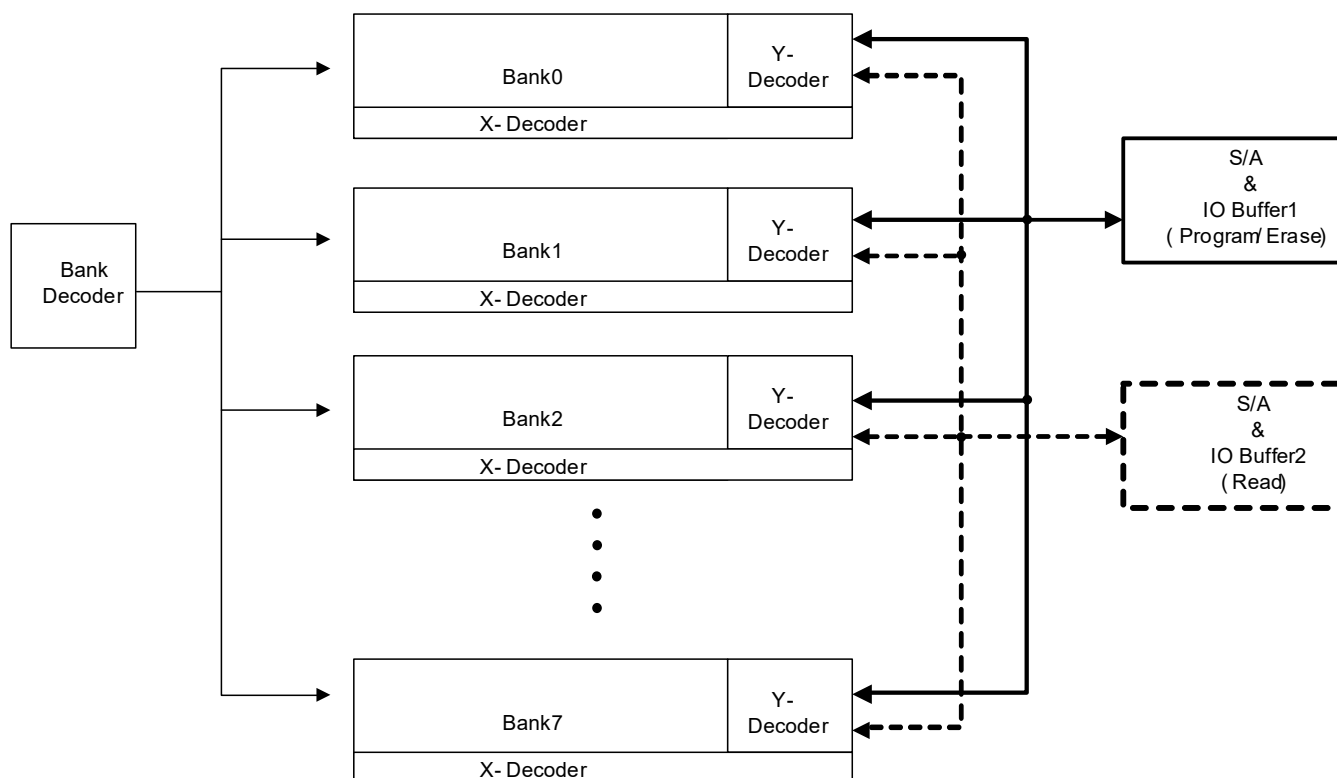
Figure 8.33 Block Diagram while Program/Erase Operation
