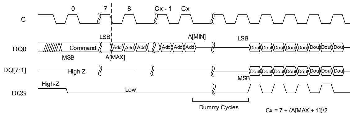
Figure 8.8 DDR OCTAL OUTPUT FAST READ with DDR ADDRESS and DATA (1S-1D-8D)– 9Dh (3)
