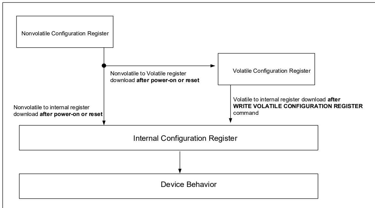
Figure 6.1 Internal Configuration Register
