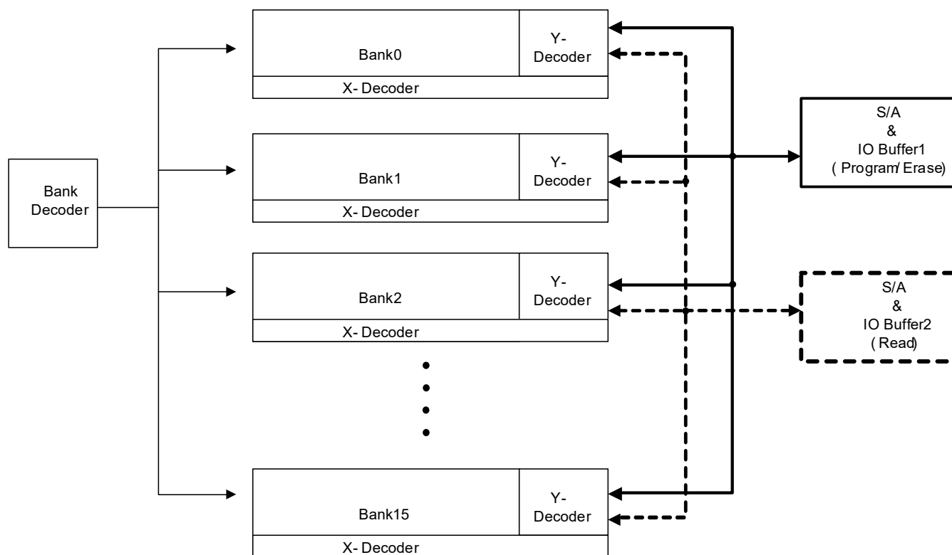
Figure 8.33 Block Diagram while Program/Erase Operation
