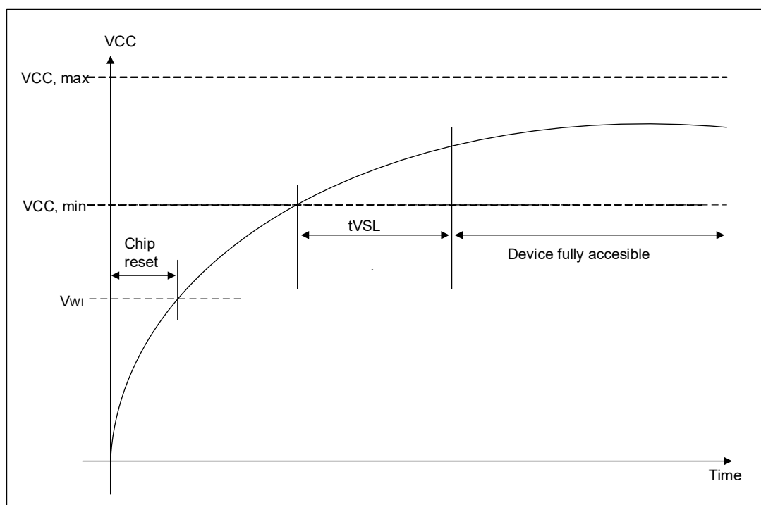
Figure 8.26 Power-Up Timing
