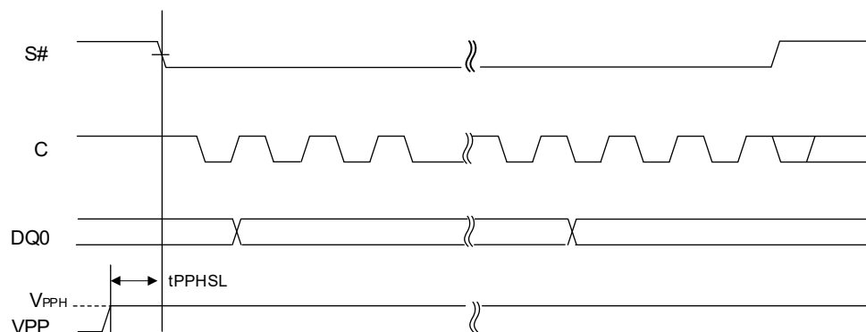
Figure 9.9 V_{PPH} Timing
