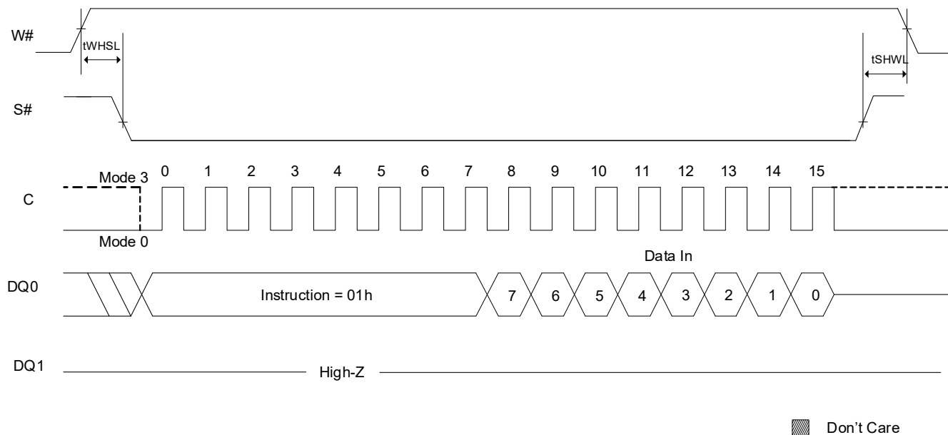
Figure 9.6 Output Timing - SDR
