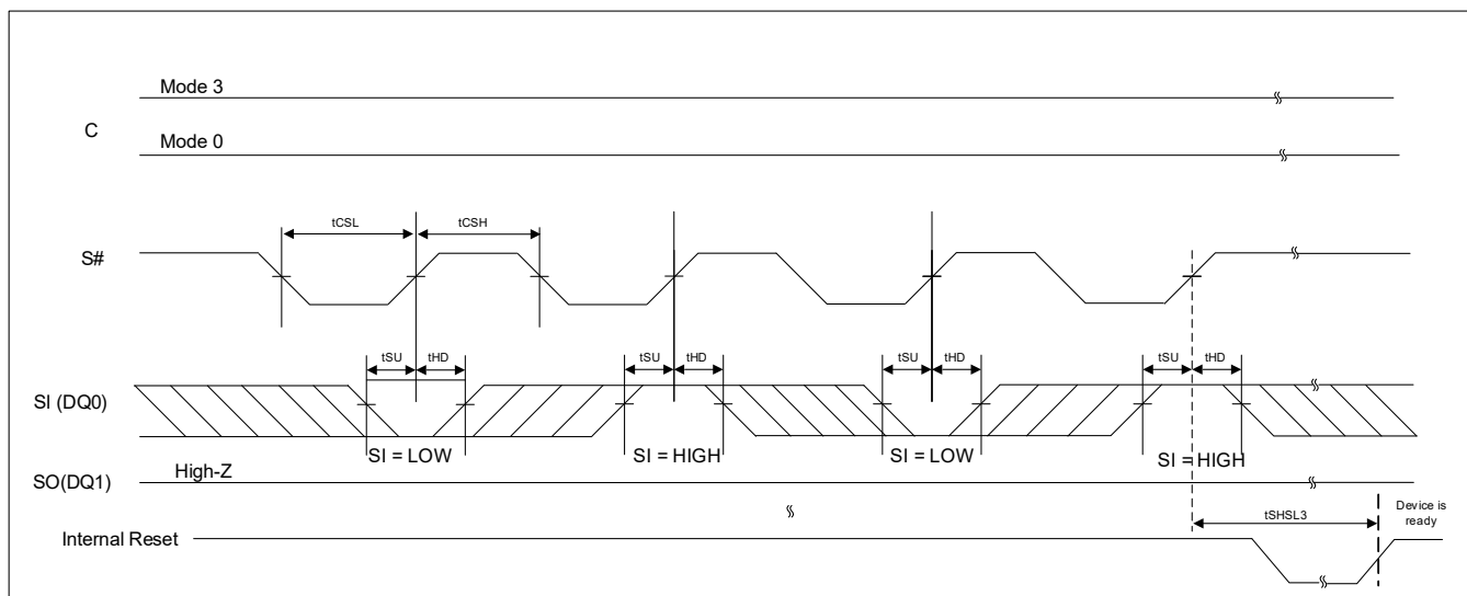
Figure 8.32 Timing for In-Band RESET Operation
