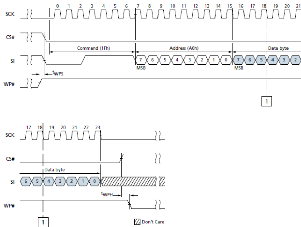
Figure 4.3 WP# Timing
