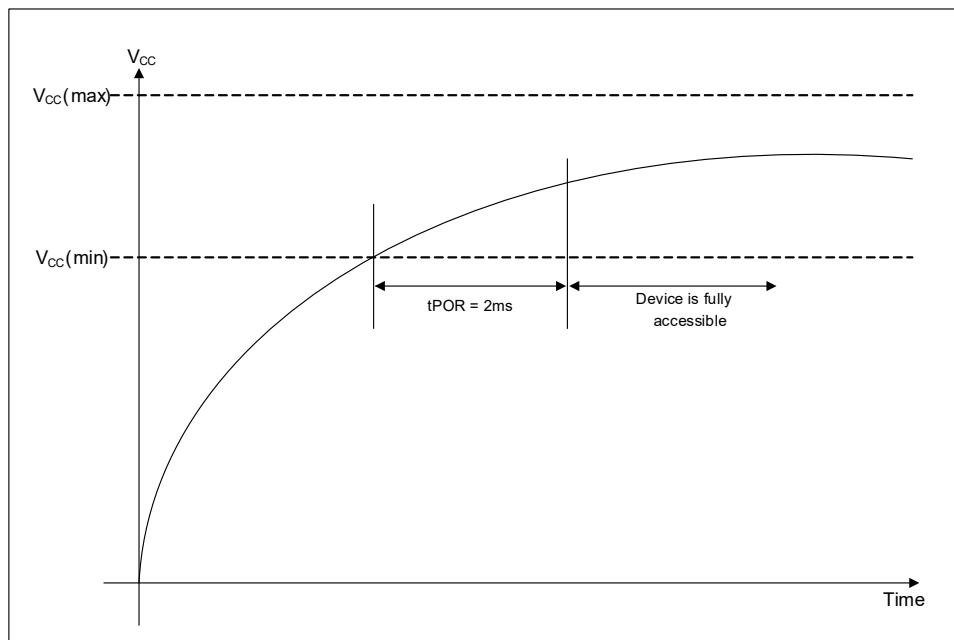
Figure 8.1 Power-Up Sequence
