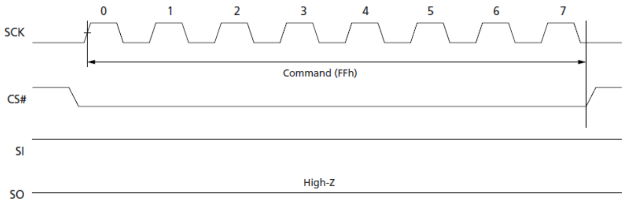
Figure 8.2 RESET (FFh) Timing
