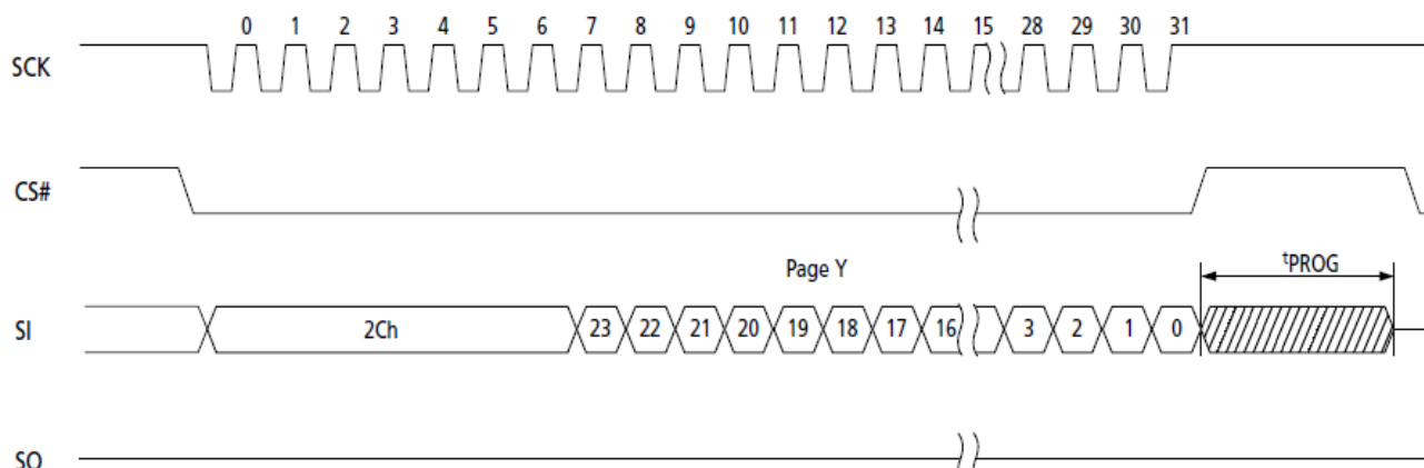
Figure 6.1 PROTECT command Cycle
