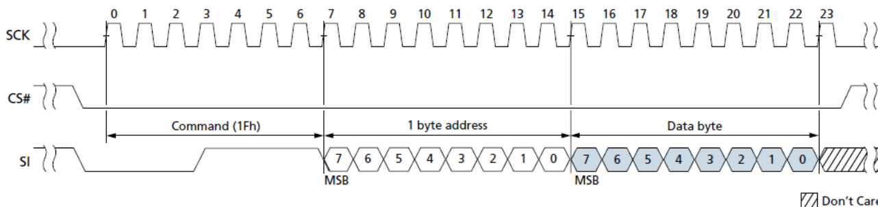
Figure 3.2 SET FEATURE (1Fh) Timing
