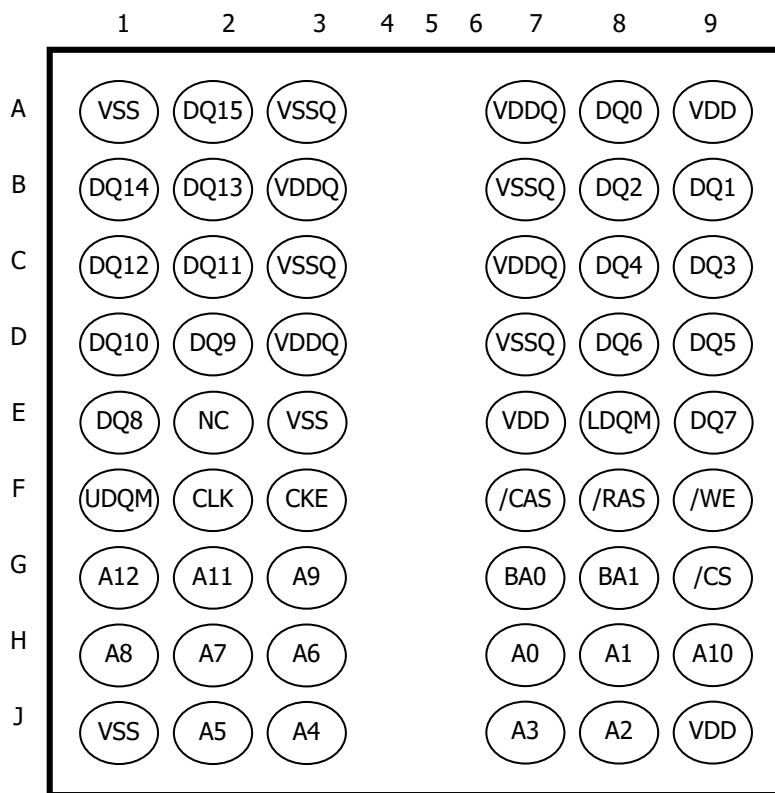
Figure 1: 54Ball BGA Ball Assignment
