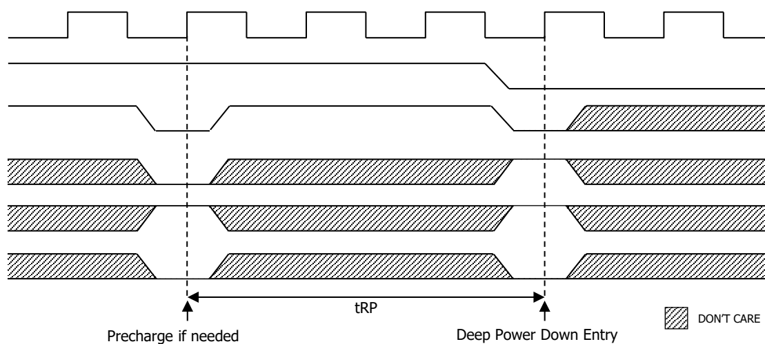
Figure 7: Deep Power Down Mode Entry
