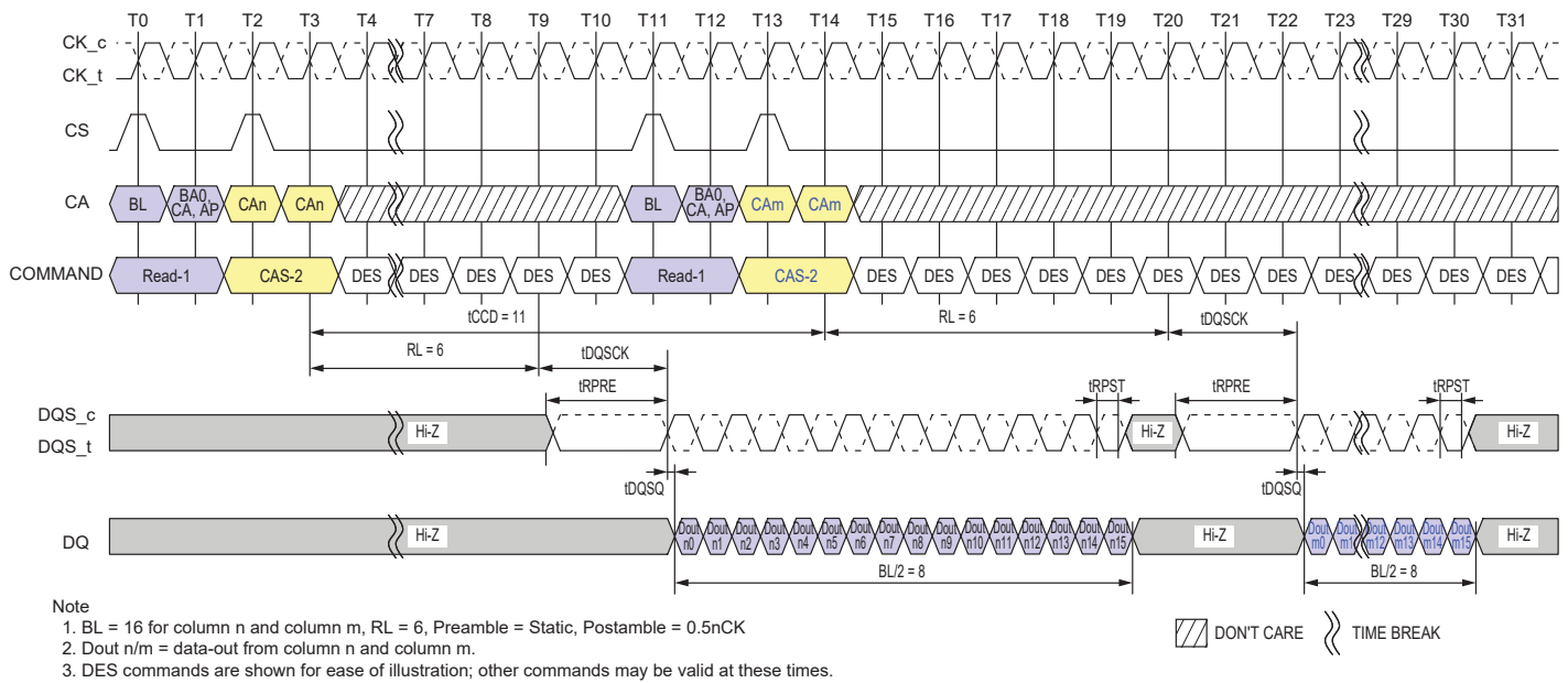
Figure 4.31 — Consecutive Reads Operation: tCCD = Min +3, Preamble = Static, 0.5nCK Postamble
