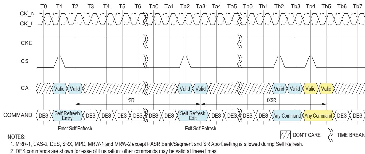
Figure 4.56b — Self Refresh Entry/Exit Timing
