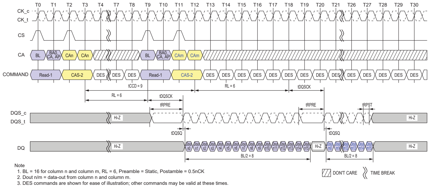
Figure 4.23 — Consecutive Reads Operation: t_{CCD} = \text{Min} +1 , Preamble = Static, 0.5nCK Postamble
