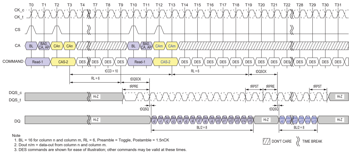
Figure 4.24 — Consecutive Reads Operation: t_{CCD} = \text{Min} +2 , Preamble = Toggle, 1.5nCK Postamble
