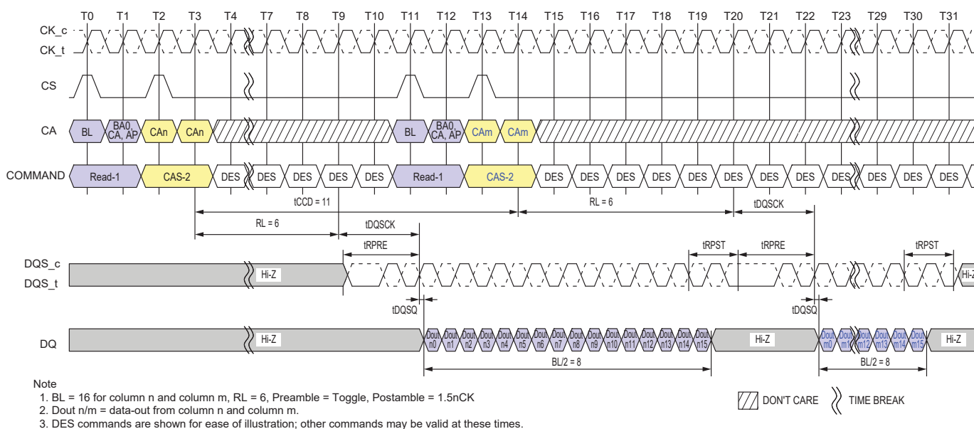
Figure 4.28 — Consecutive Reads Operation: t_{CCD} = \text{Min} +3 , Preamble = Toggle, 1.5nCK Postamble
