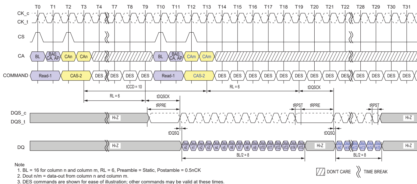
Figure 4.27 — Consecutive Reads Operation: t_{CCD} = \text{Min} +2 , Preamble = Static, 0.5nCK Postamble
