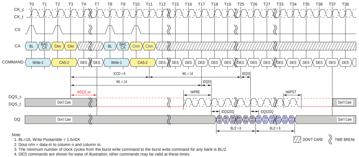
Figure 4.34 — Seamless Writes Operation: t_{CCD} = \text{Min}, 1.5nCK Postamble
