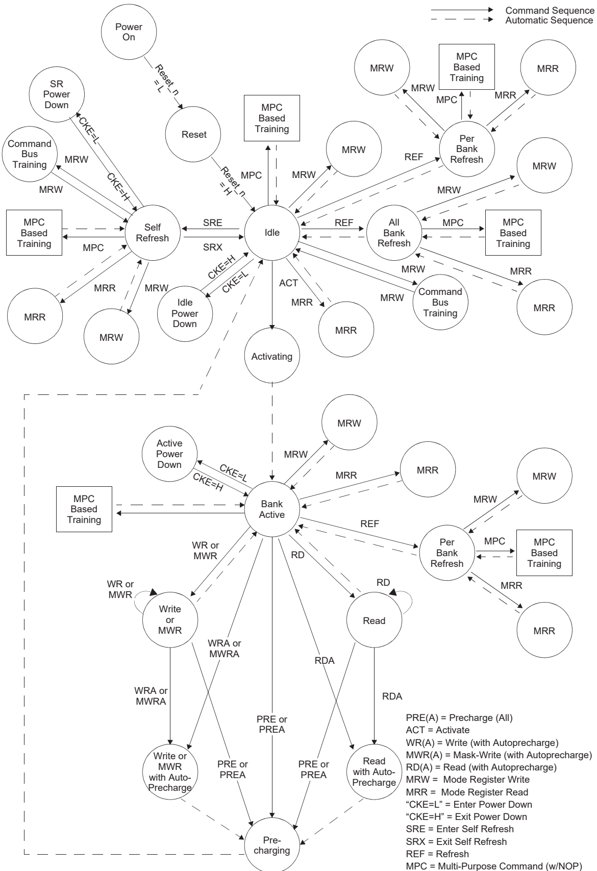
Figure 3.2 — LPDDR4: Simplified Bus Interface State Diagram - 1
