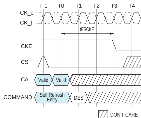
Figure 4.59 — tESCCKE Timing
