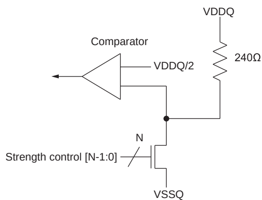
Figure 7.19 — Pull-down calibration
