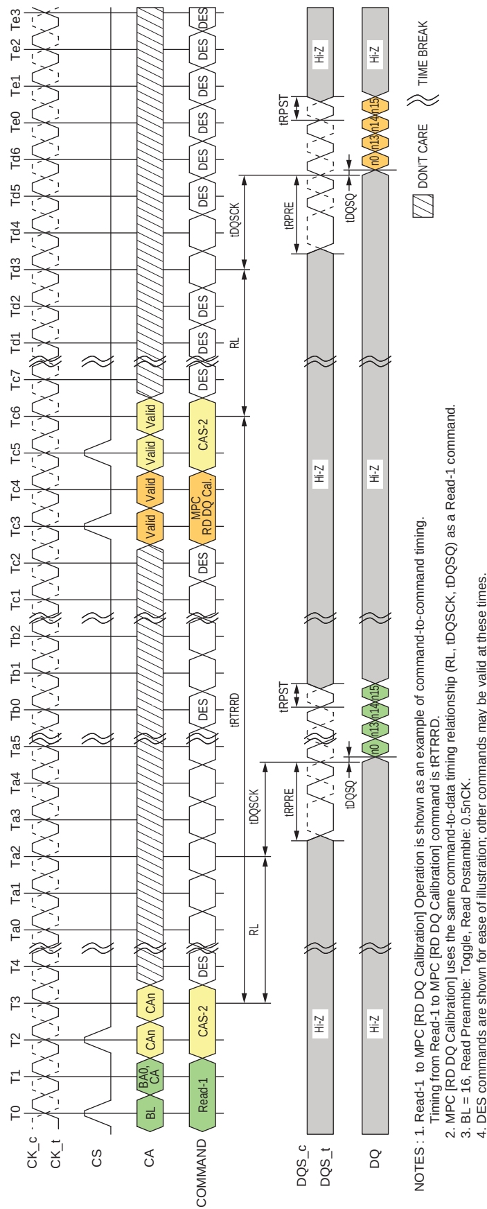
Figure 4.95 — DQ Read Training Timing: Read to Read DQ Calibration
