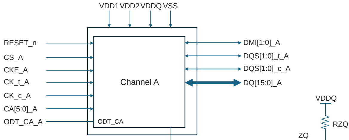
Figure 3.1 – Single-channel (x16) Package Diagram
