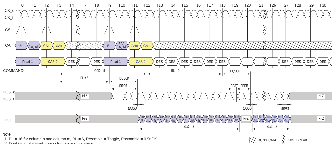
Figure 4.21 — Consecutive Reads Operation: tCCD = Min +1, Preamble = Toggle, 0.5nCK Postamble
