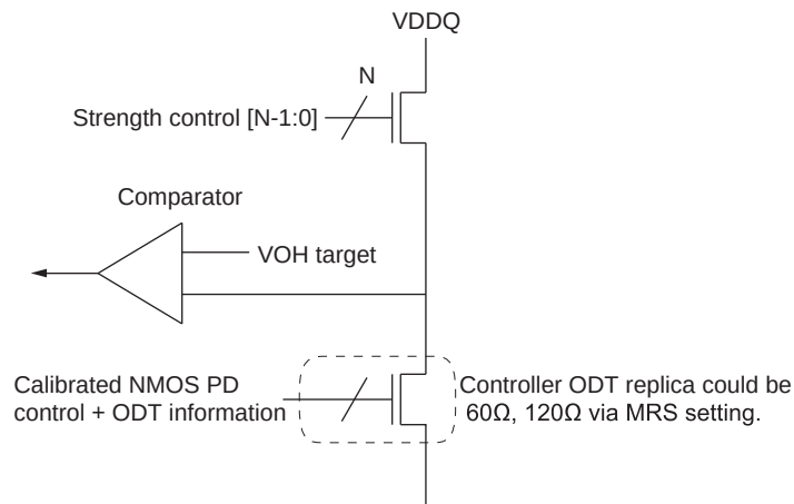
7.20 — pull-up calibration
