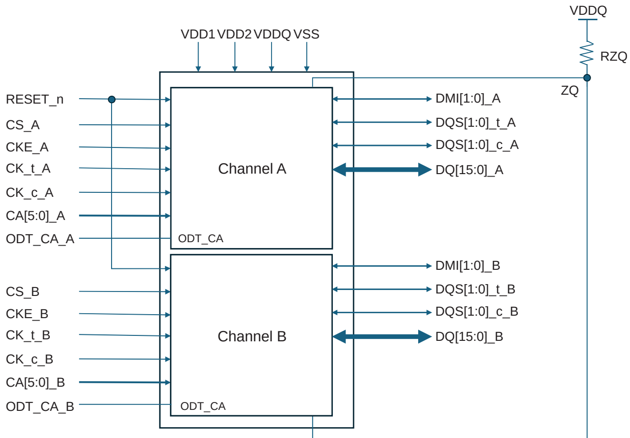
Figure 3.1 – Dual-channel (x32), Single-rank Package Diagram
