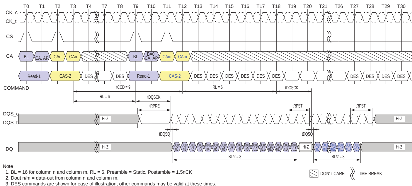
Figure 4.22 — Consecutive Reads Operation: t_{CCD} = \text{Min} + 1 , Preamble = Static, 1.5nCK Postamble
