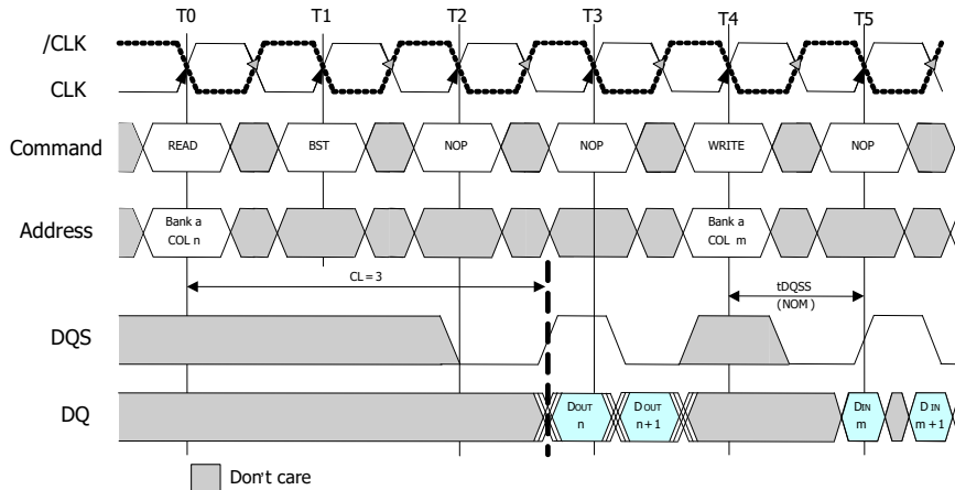
Figure 19: Read to write terminate (BL=4,8 or 16)
