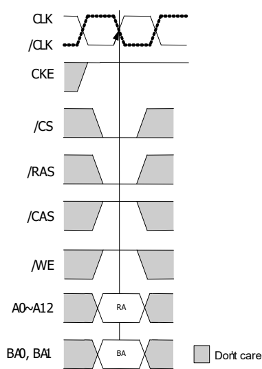
Figure 11: Active command
