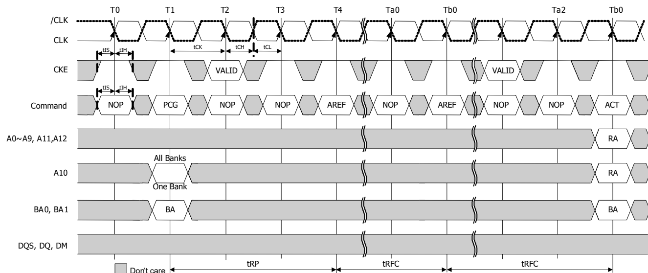
Figure 34: Auto refresh
