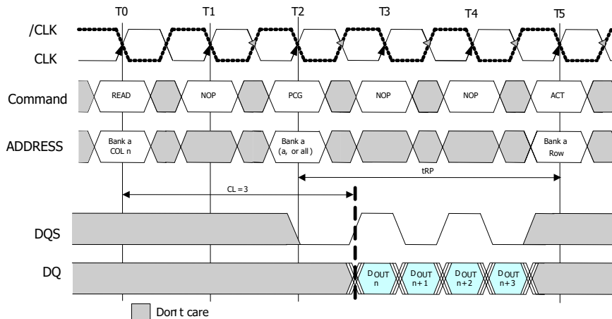
Figure 20: Read to Precharge (BL=4)
