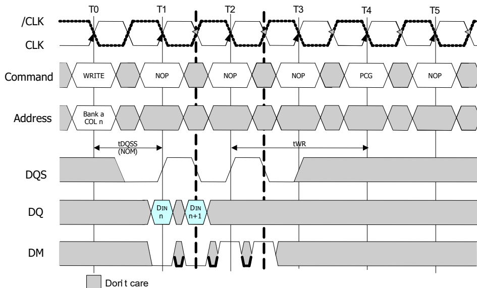
Figure 30: Write to Precharge (Interrupting)
