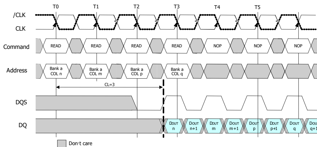
Figure 17: Random Read access
