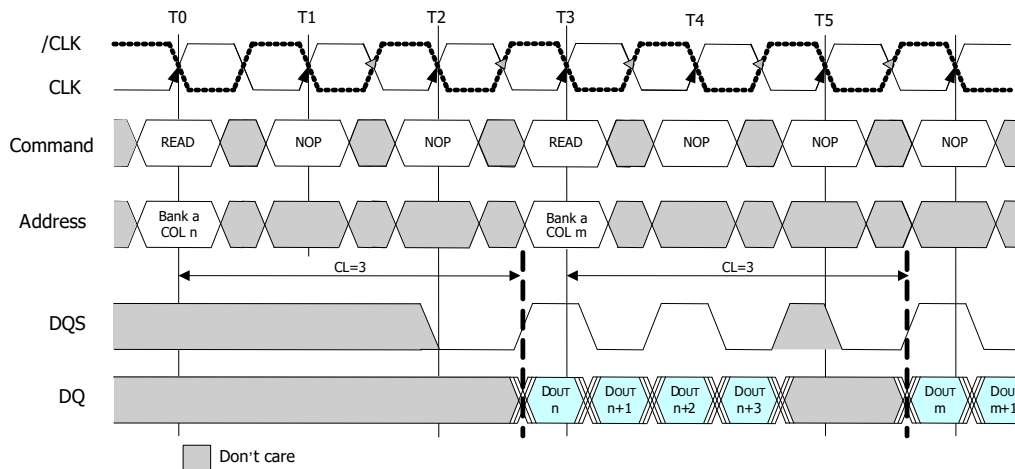
Figure 16: Non-Consecutive Read bursts (BL=4)
