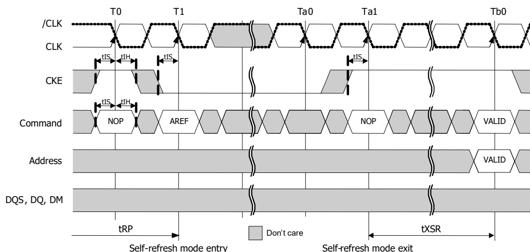
Figure 35: Self refresh
