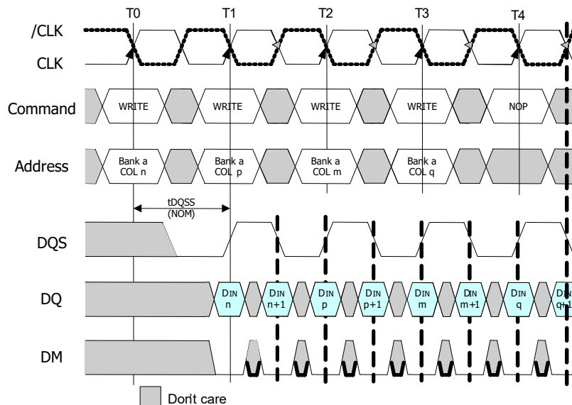
Figure 25: Random Write to write
