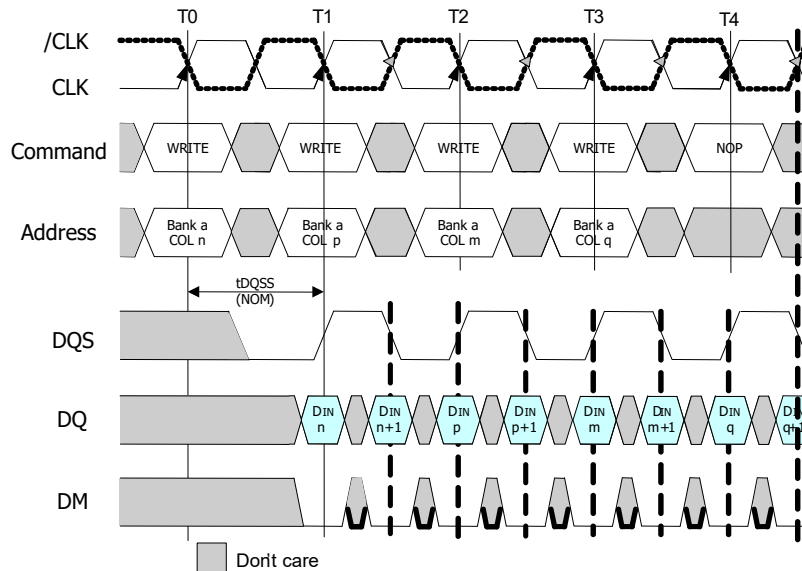
Figure 25: Random Write to write
