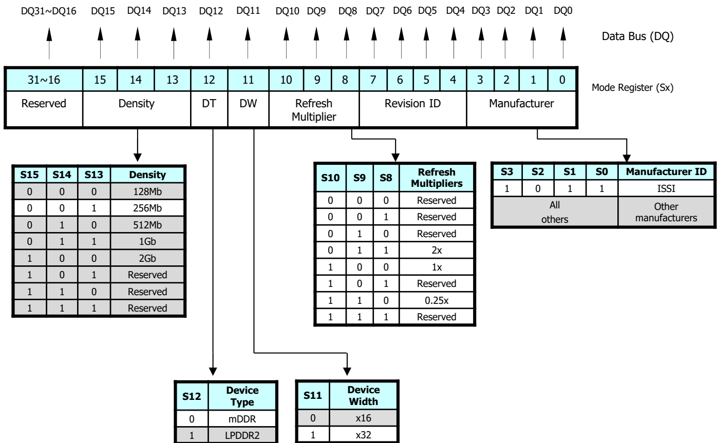
Figure 8: Status Register Read (SRR)
