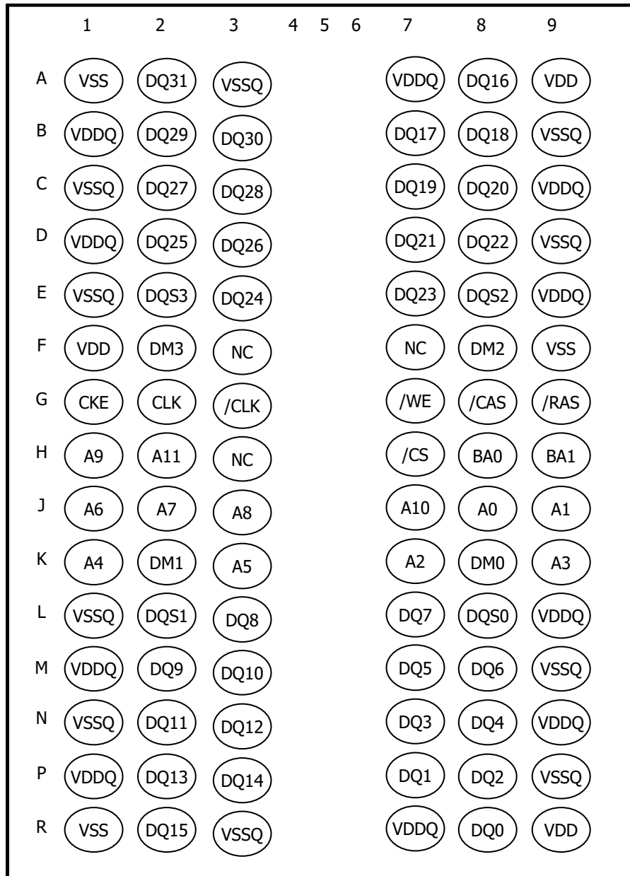
Figure 1: 90Ball BGA Ball Assignment
