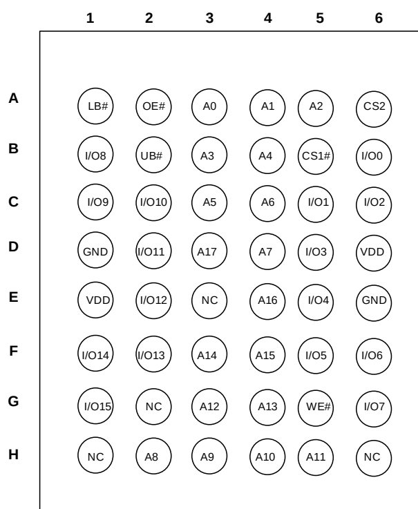
48-Pin mini BGA (6mm x 8mm),2CS, ERR1/ERR2
