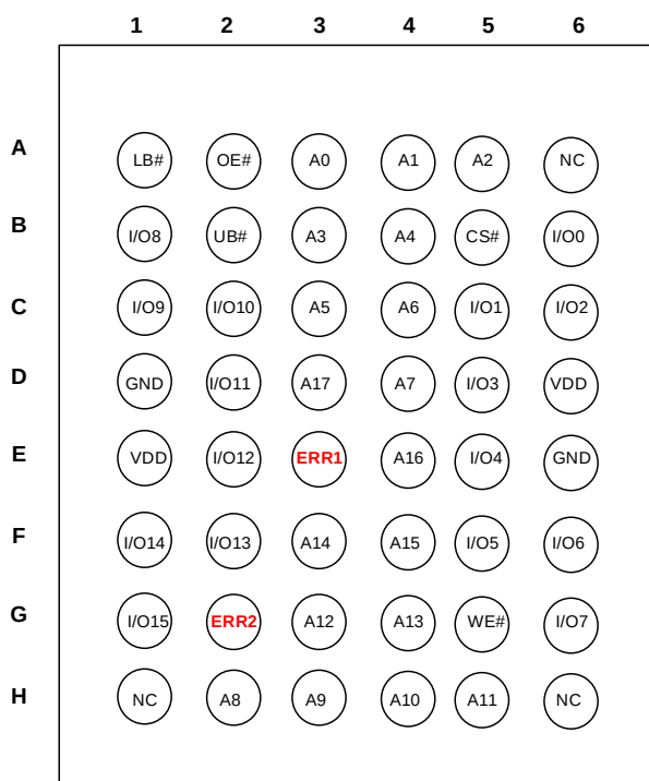
48-Pin mini BGA (6mm x 8mm),1CS, ERR1/ERR2
