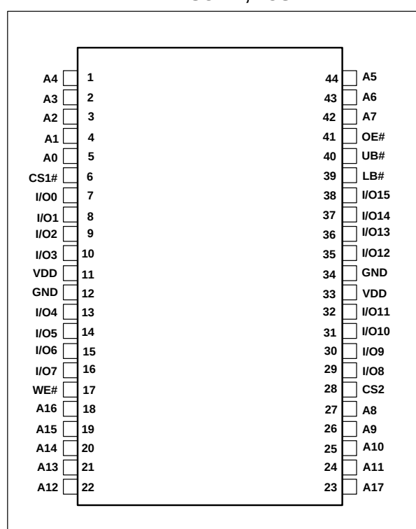
44-Pin TSOP-II, 2CS
