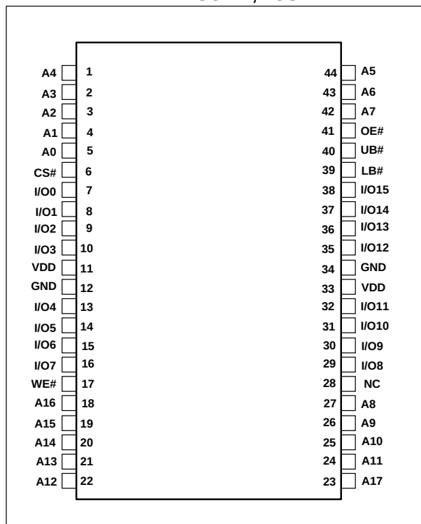
44-Pin TSOP-II, 1CS
