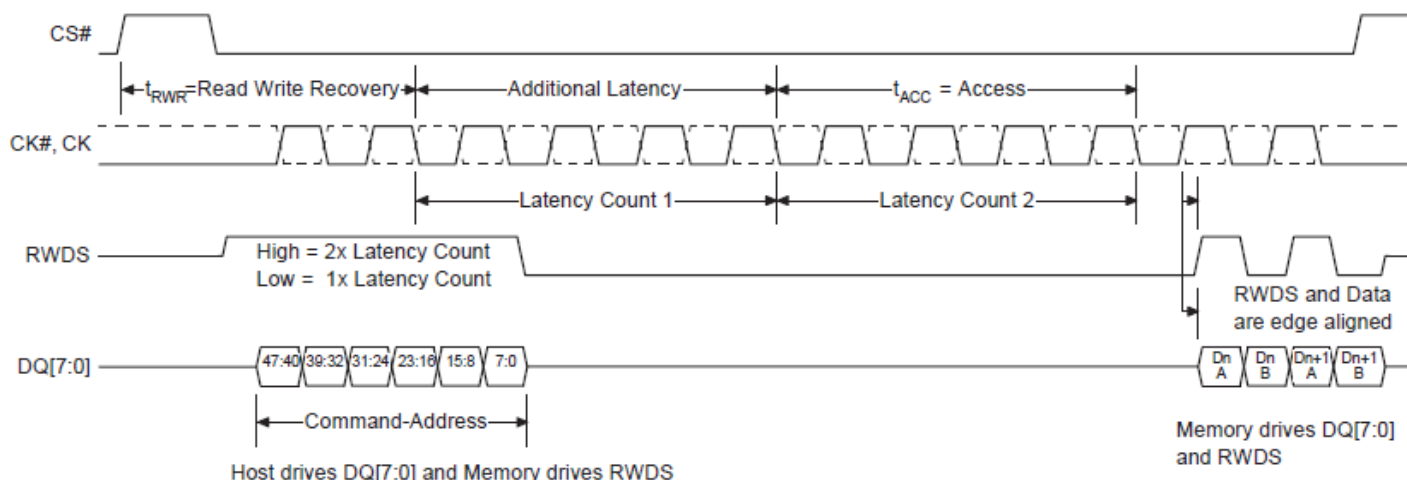
Figure 1.1 Read Transaction, Fixed Latency mode (1)
