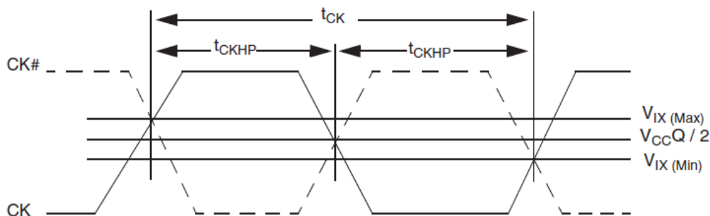
Figure 10.3 Clock Characteristics
