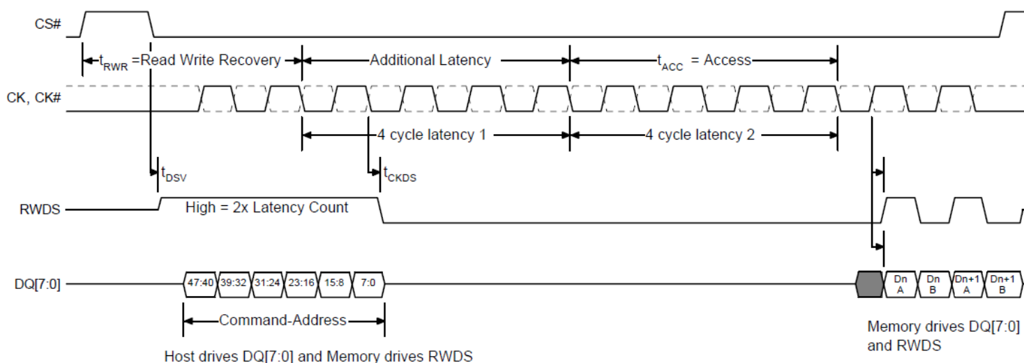
Figure 3.4 Read Transaction with Fixed Latency mode.
