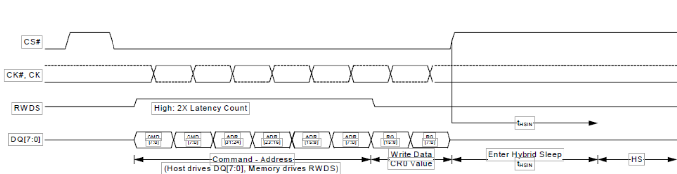
Figure 6.2 Enter HS transaction
