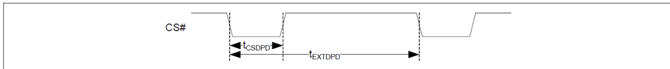
Figure 6.5 Exit DPD transaction
