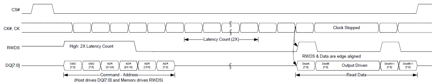
Figure 6.1 Active clock stop during read transaction (DDR)
