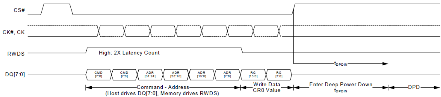
Figure 6.4 Enter DPD transaction
