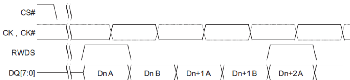
Figure 3.3 Data Placement During a Write Transaction
