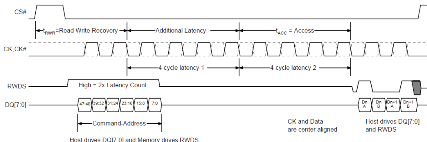
Figure 1.2 Write Transaction, Fixed Latency mode (1)
