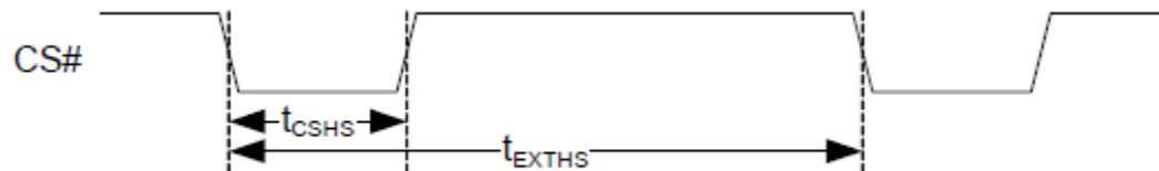
Figure 6.3 Exit HS transaction
