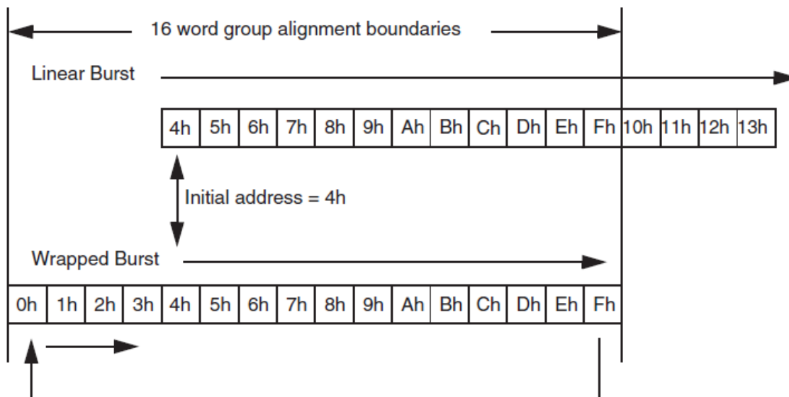
Figure 1.3 Linear Versus Wrapped Burst Sequence
