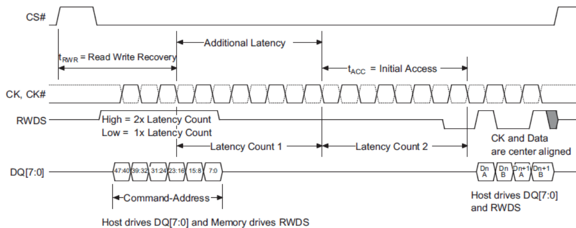
Figure 3.5 Write Transaction with Fixed Latency mode
