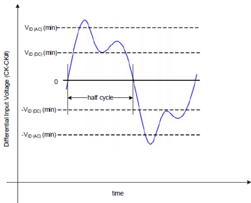
Figure 10.4 Differential clock (CK/CK#) input swing
