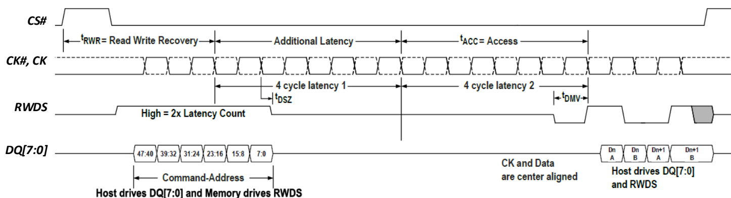
Figure 10.8 Write Timing Diagram — With Additional Latency
