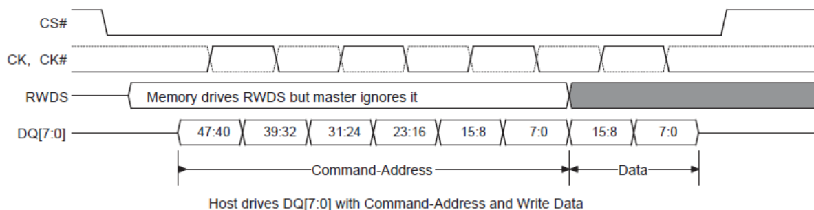
Figure 3.6 Register Write Operation without Initial Latency
