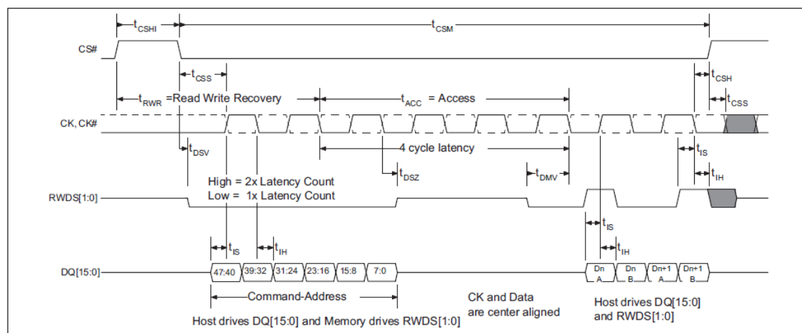
Figure 10.8 Write Timing Diagram — No Additional Latency
