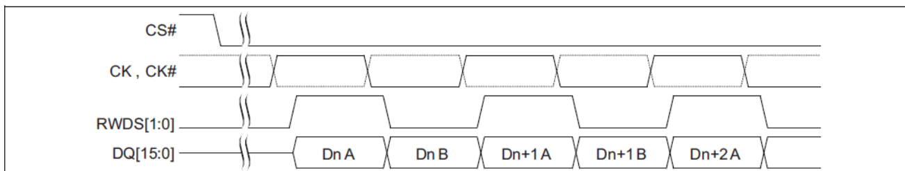
Figure 3.2 Data Placement During a Read Transaction
