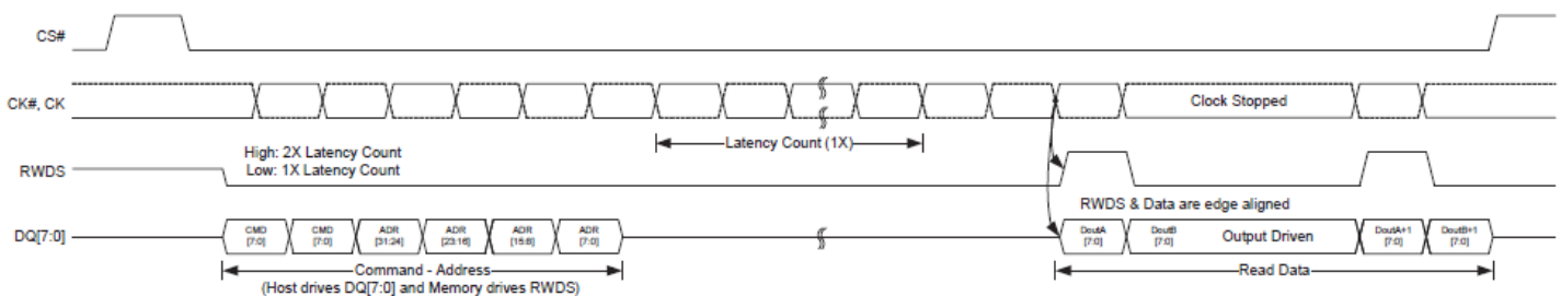
Figure 6.1 Active Clock Stop During Read Transaction (DDR) (1)
