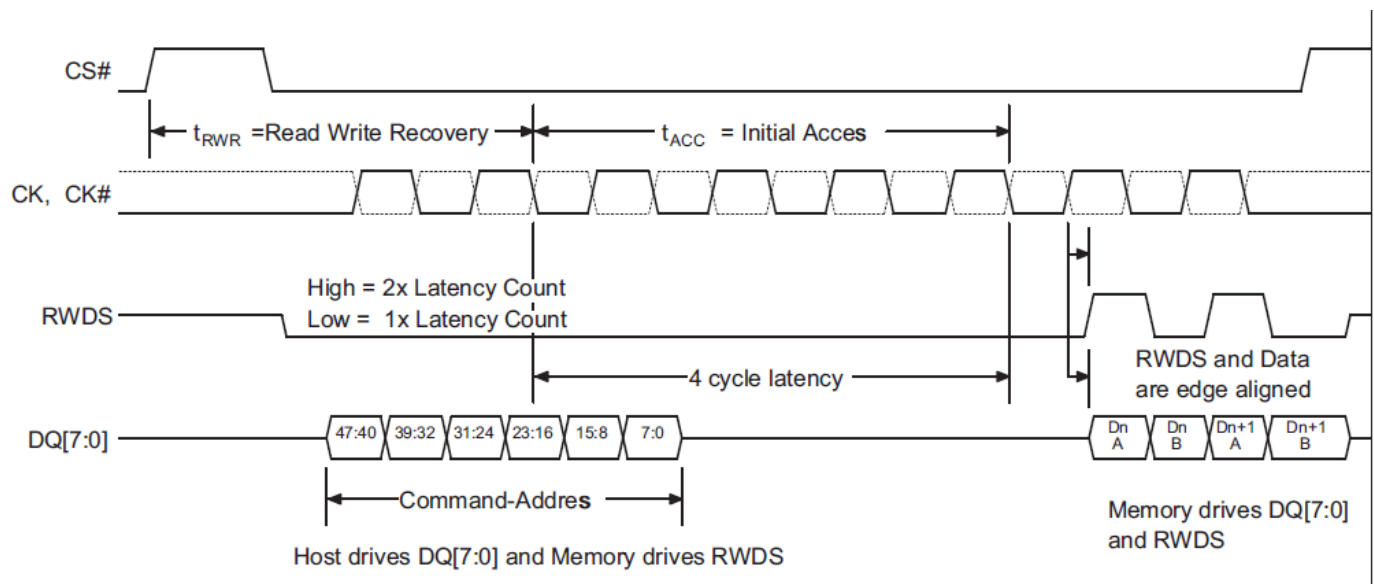
Figure 3.4 Read Transaction with additional Initial Latency
