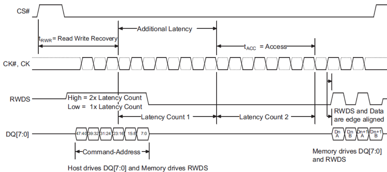
Figure 3.5 Read Transaction Without Additional Initial Latency
