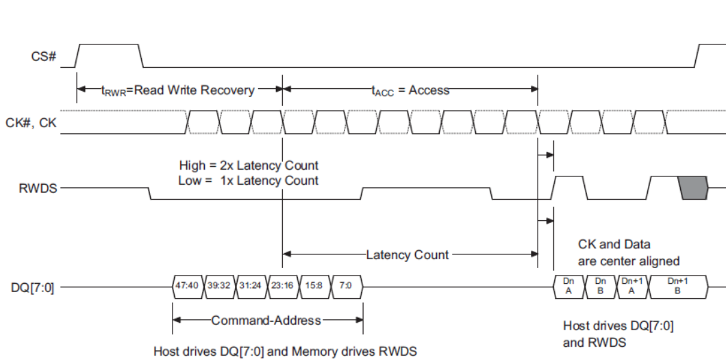
Figure 3.7 Write Transaction without Additional Initial Latency
