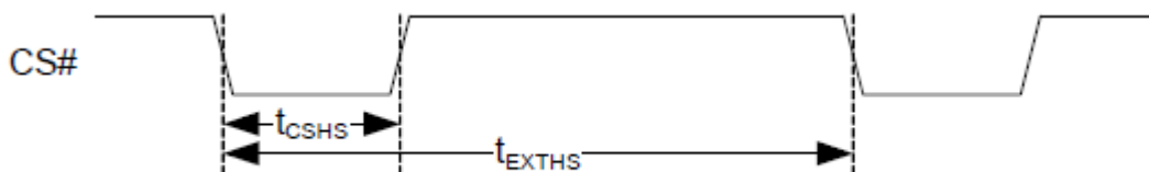
Figure 6.3 Exit HS transaction
