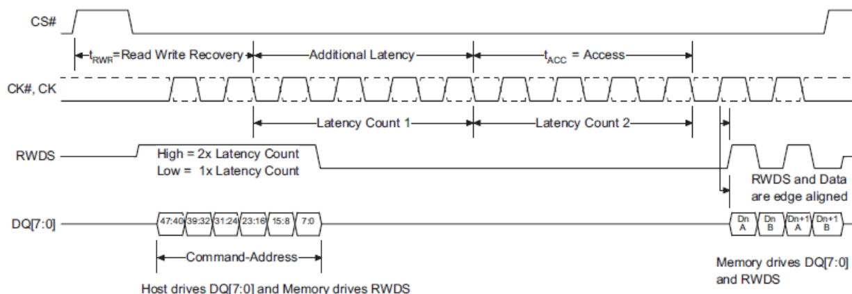
Figure 1.2 Read Transaction, Additional Latency Count
