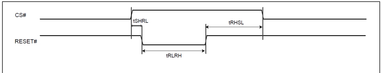
Figure 5.8 RESET Timing
