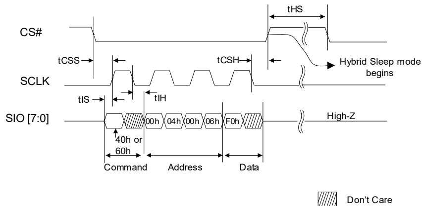
Figure 6.6 Hybrid Sleep Mode Entry Timing Diagram
