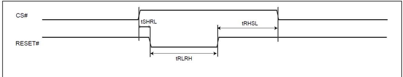
Figure 5.10 RESET Timing
