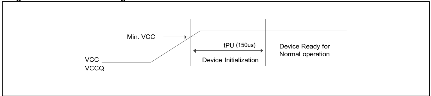
Figure 5.9 POWER-UP Timing
