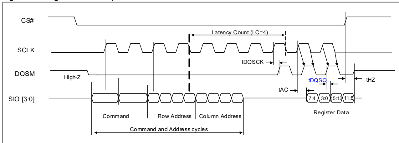
Figure 6.2 Register READ Operation
